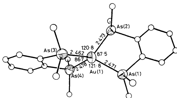
FIGURE 1 The [\text{Au}(\text{pdma})_2]^+ cation showing bond lengths (Å, \pm 0.002 ) and angles ( ^\circ , \pm 0.2 ) at the gold atom. The C atoms are plotted as circles, rather than thermal ellipsoids, for clarity; H atoms are omitted. Other angles: As(1)-Au(1)-As(3) 123.0, As(2)-Au(1)-As(4) 121.1°
