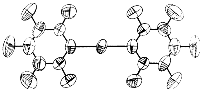
FIGURE 2 One of the two [\text{Au}(\text{C}_6\text{F}_5)_2]^- anions. Au-C bond lengths: are 2.04 (here), 2.06 Å ( \pm 0.02 Å)
